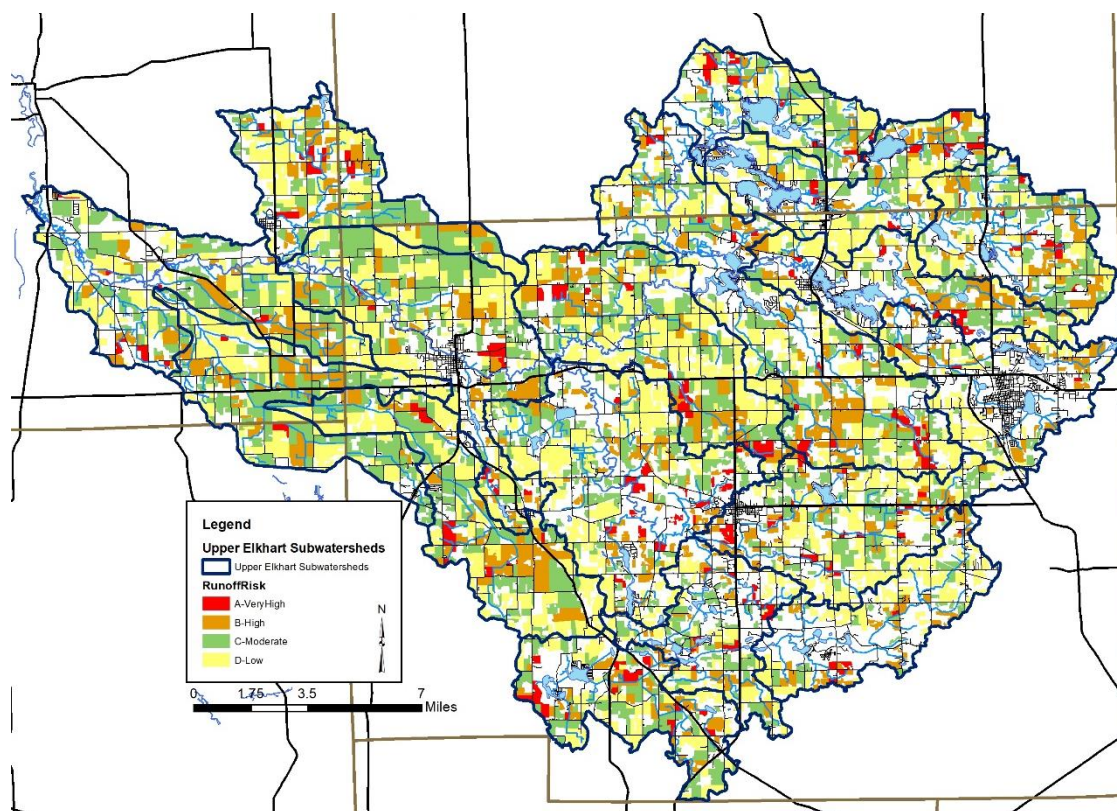
Figure 112. Runoff risk ratio developed using ACPF for the Upper Elkhart River Watershed.
