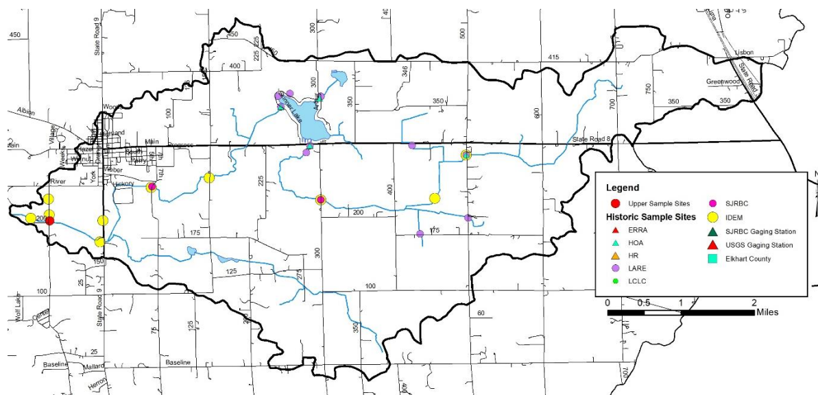
Figure 87. Locations of historic and current water quality data collection and impairments in the Skinner Lake-Croft Ditch subwatershed.
