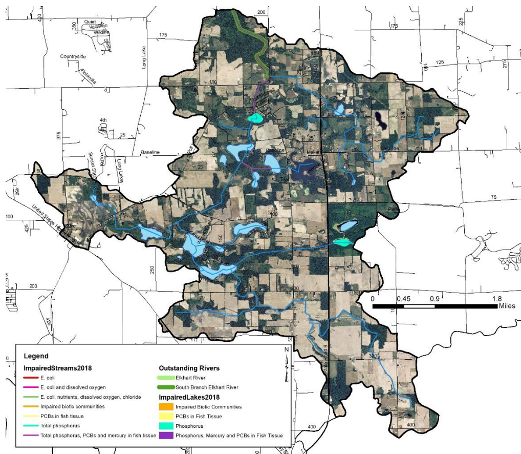
Figure 88. Muncie Lake-South Branch Elkhart River subwatershed.
