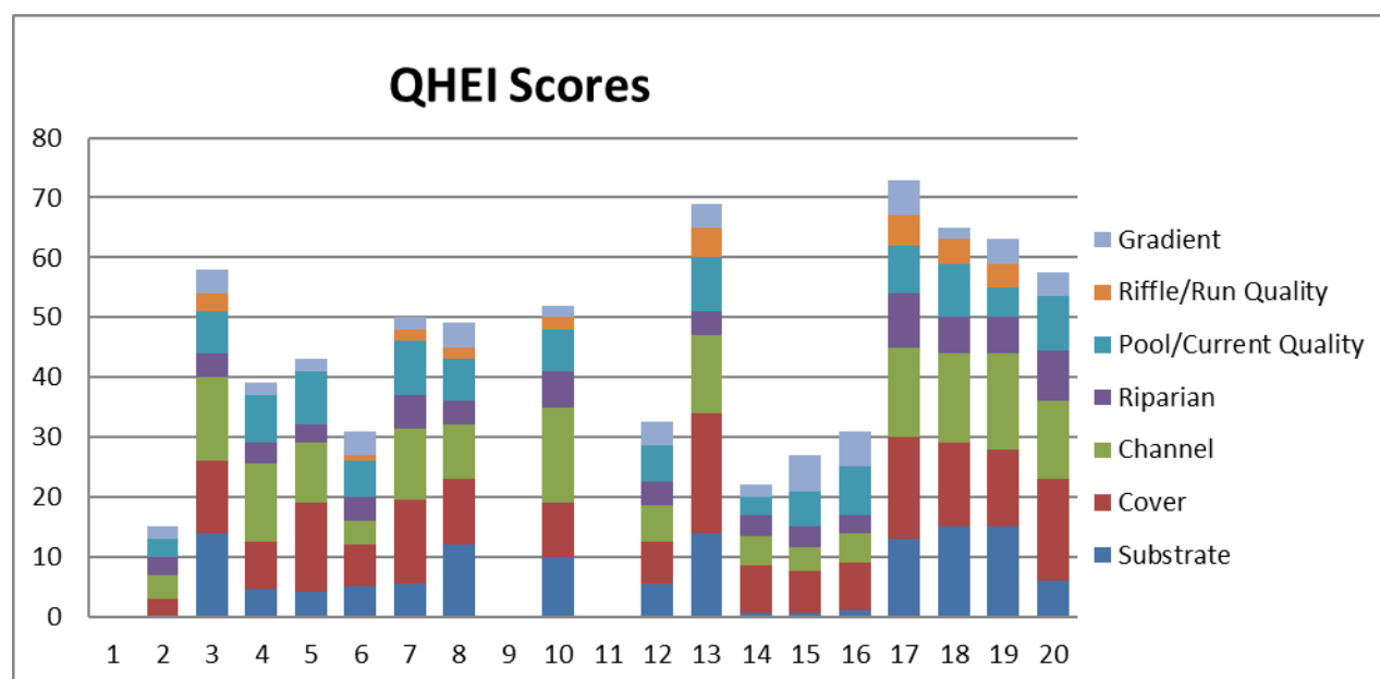
Figure 54. Cumulative metrics used to calculate QHEI scores for Upper Elkhart River Watershed streams in 2022.
