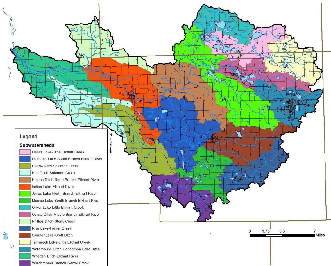
Figure 57. 12-digit Hydrologic Unit Codes subwatersheds in the Upper Elkhart River Watershed.
